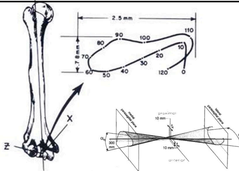
FIG. 5 Configuration and dimensions of the locus of the instant centers of rotation of the elbow *.
